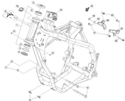
TAV.31 Telaio - Frame - Chassis - Rahmen - Chasis
